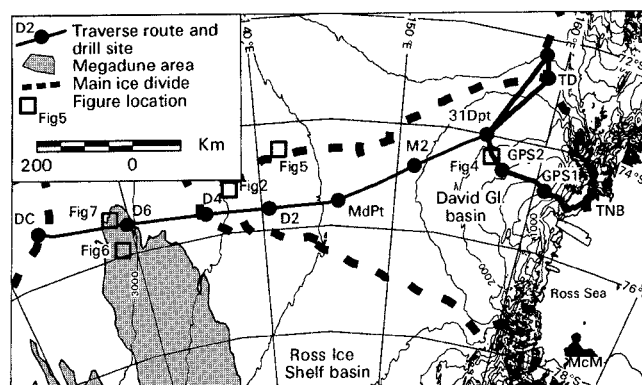
Fig. 1. Schematic map of the PNRA-ITASE traverse route, including firm-core location (drill sites), megadune area, main ice divide and figure locations. 31Dpt, 31 Deposit; DC, Dome C; McM, McMurdo; MdPt, Midpoint; TNB, Terra Nova Bay station; TD, Talos Dome.
