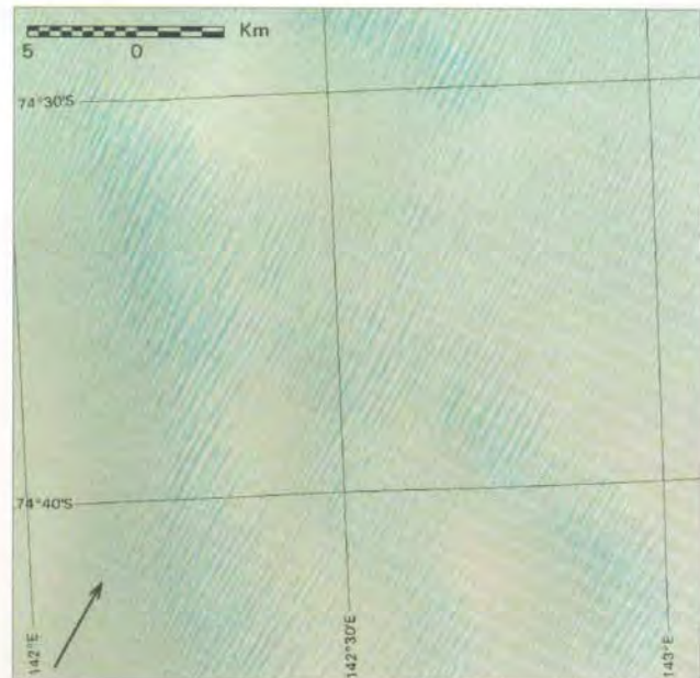
Fig. 5. Subscene of Landsat TM image in false colour (RGB, 4, 3, 2) showing an area of plateau with a sastrugi glazed surface field; the arrow shows the prevailing wind direction.
