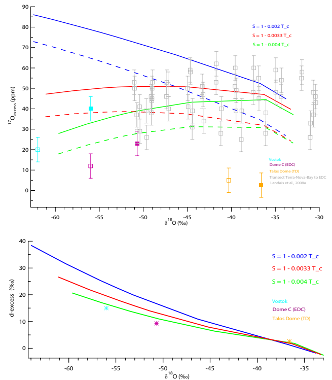
Fig. 3. Dependency of ^{17}\text{O} -excess ( a ), upper panel on supersaturation S as a function of \delta^{18}\text{O} (with fixed climatic parameters, \text{RH}_n , T_{\text{source}} and T_{\text{site}} ). The different coloured lines represent different S . The dashed lines represent S , but with 10 times more re-evaporation ( \gamma ) of the liquid phase in the cloud. The filled symbols are the EH values and the empty ones are the LGM values of ^{17}\text{O} -excess (analytical uncertainty = \pm 6 ppm). The light grey dots are the data of the transect study from Terra Nova Bay to EDC (Landais et al., 2008a). ( b ) (lower panel): dependency of d -excess on S as a function of \delta^{18}\text{O} (with fixed climatic parameters, \text{RH}_n , T_{\text{source}} and T_{\text{site}} ). The coloured lines represent different S . Data points (star-symbols) for EH stem from (EPICA Members, 2004; Stenni et al., 2010, 2004, 2001; Vimeux et al., 1999)
