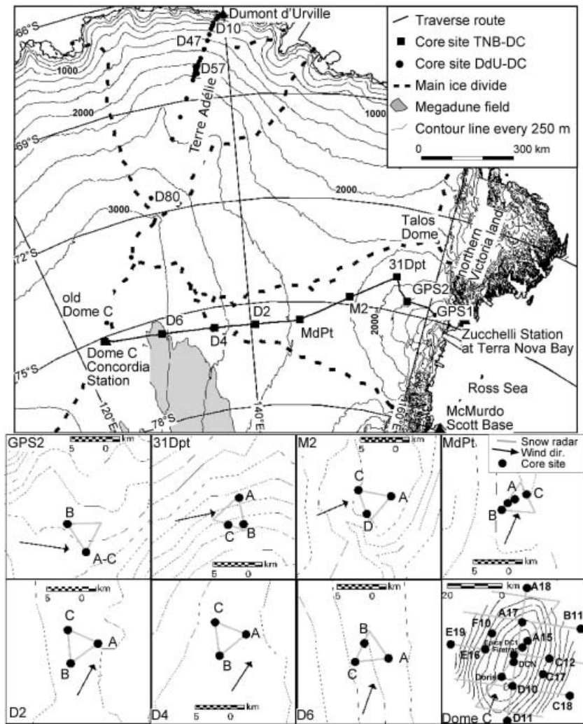
Fig. 1. Schematic map of the traverse from TNB to DC and site locations, and detailed maps of drill sites (contour every 10 m for GPS2, 31Dpt, M2, MdPt, D2, D4, D6, from Rémy and others, 1999); contour every 1 m for DC, from Capra and others (2000); prevalent wind direction from Frezzotti and others (2002b).
